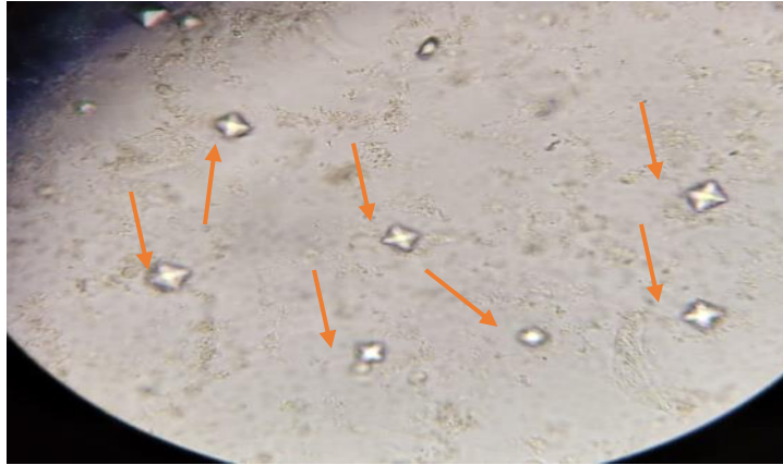
Unsur Kristal Kalsium Oksalat
