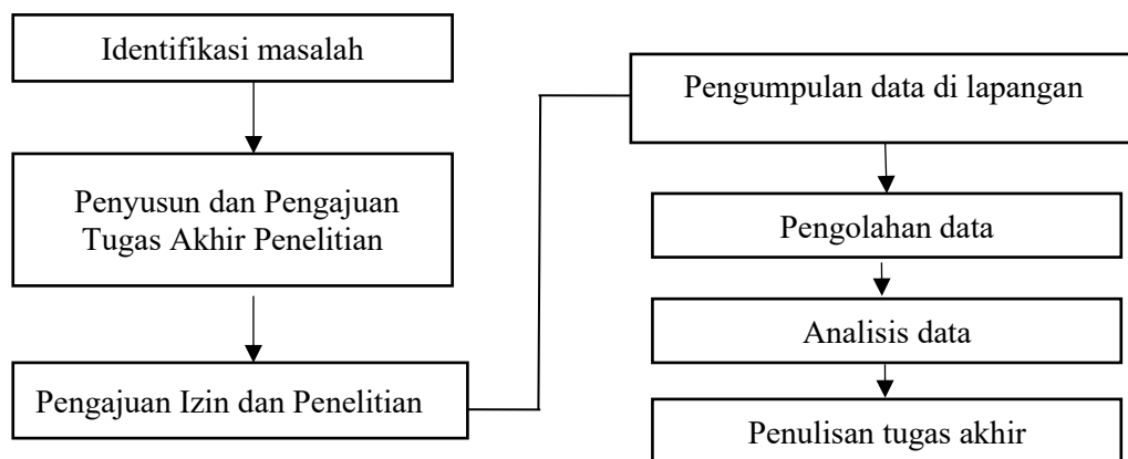
Gambar 3. Alur Penelitian
