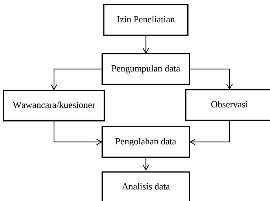
Gambar 3. Alur Penelitian
