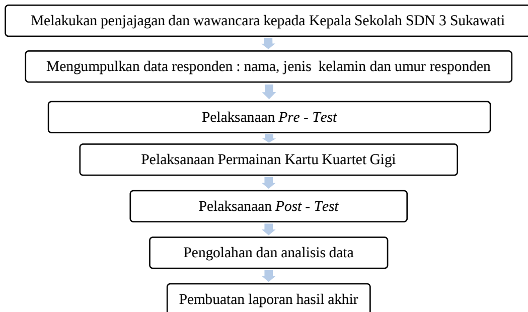
Gambar 3 Alur Penelitian
